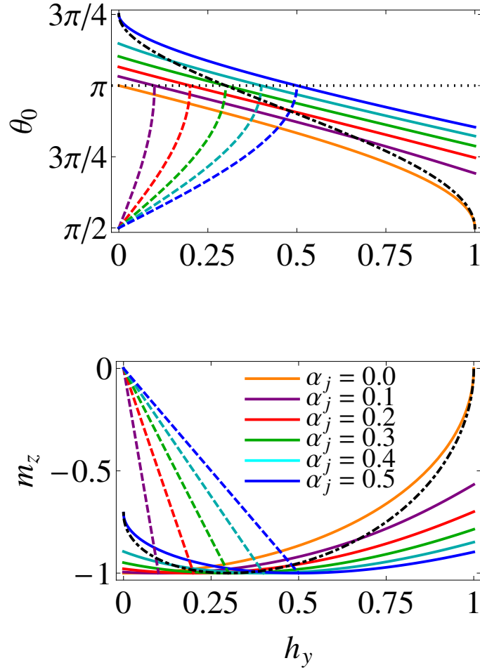
Figure 6.9: Upper panel: The polar angle \theta of the intermediate states as a function of fields for varying currents. Lower panel: The \hat{z} components of the intermediate states. The IP equilibria and OOP equilibria are represented by solid lines and dashed lines in both panels, respectively. The solid lines above \theta = \pi in the upper panel indicate the equilibria are in the -y half of the unit sphere. The IP phase diagram is plotted with dot-dashed lines in both panels.
