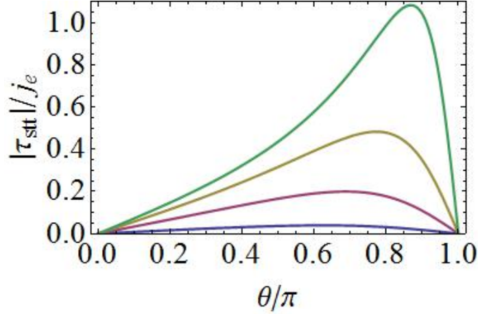
Figure 2.3: Dependence of spin transfer strength on the spin current polarization. The polarization coefficient P is set to 0.1, 0.3, 0.5 and 0.7 from bottom to top.
